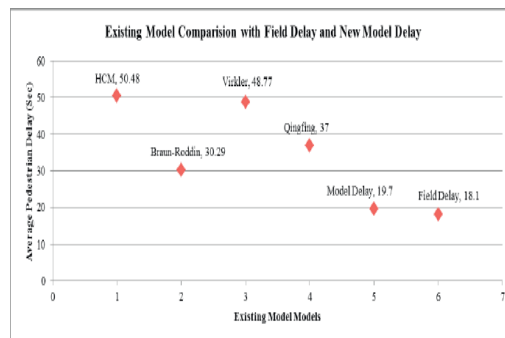
Figure 8. Existing Model Comparisons with Field Delay and New Model Delay at Holkar junction
