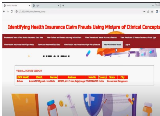
Fig.3. User details.
