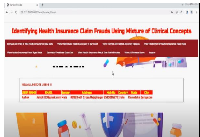
Fig.1. Home page.
