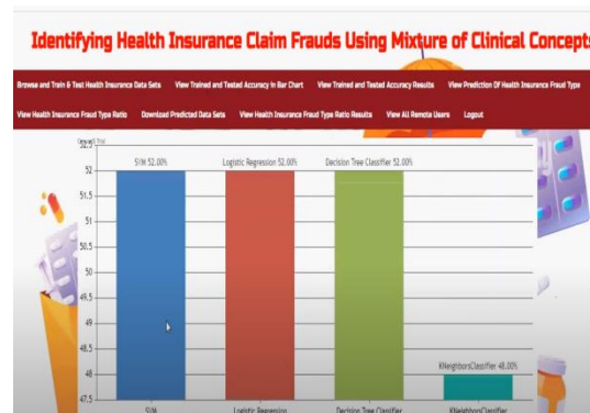
Fig.6. Output results.
