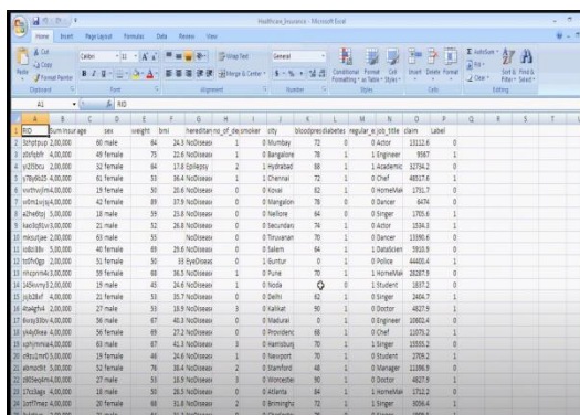
Fig.5. Dataset details.
