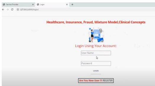
Fig.4. Login details.
